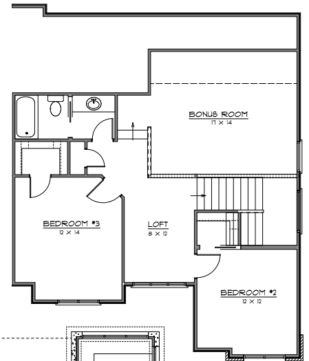
SECOND FLOOR PLAN LIVING 925 SF
